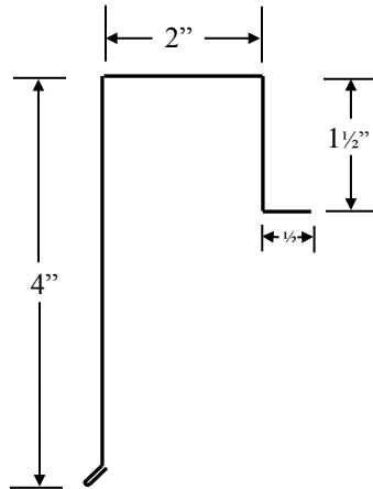
Ridge Cap
